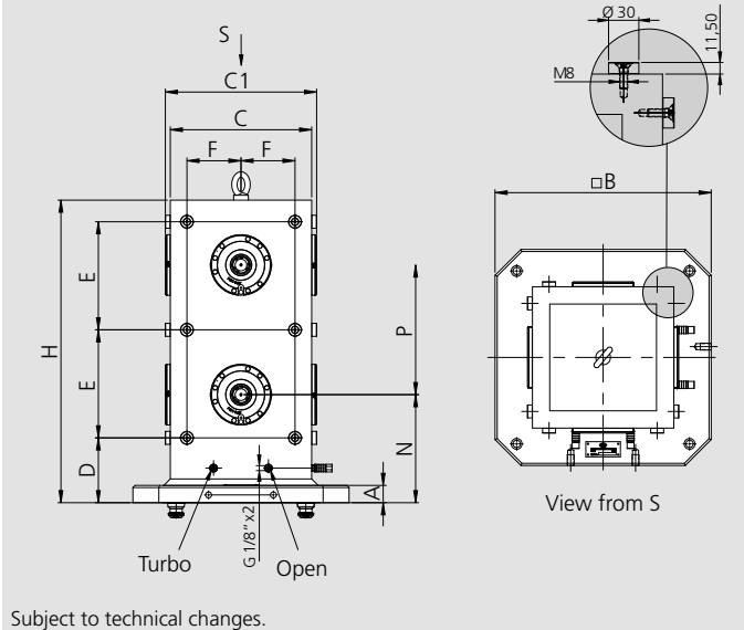
Tombstone with 8 APS modules
