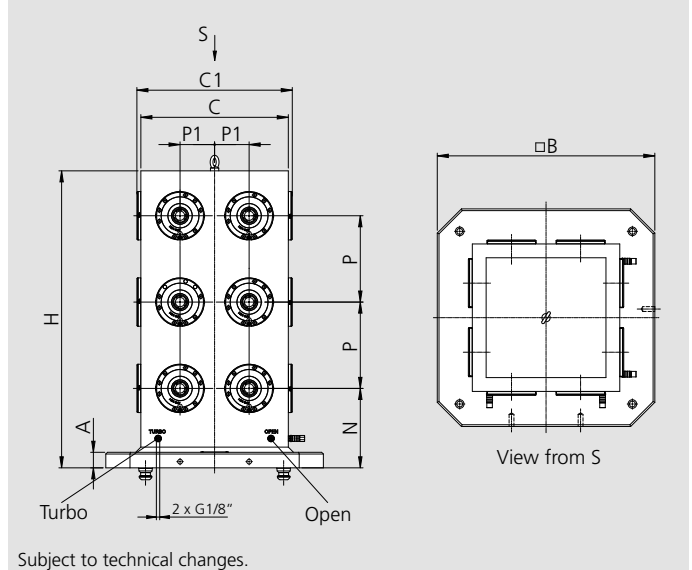
Tombstone with 24 APS modules
