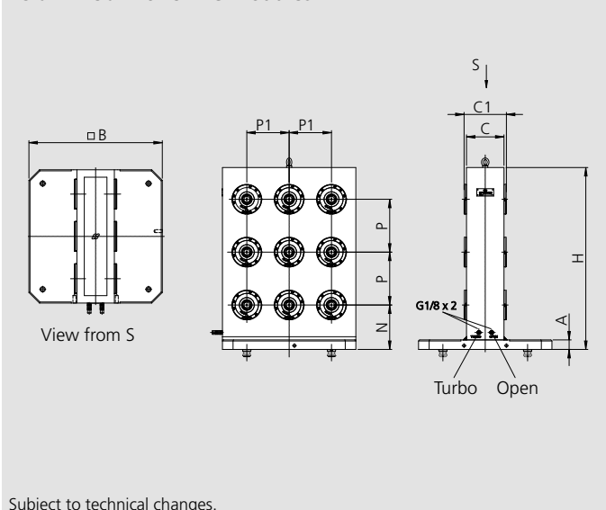
Crankweb with 8 APS modules
