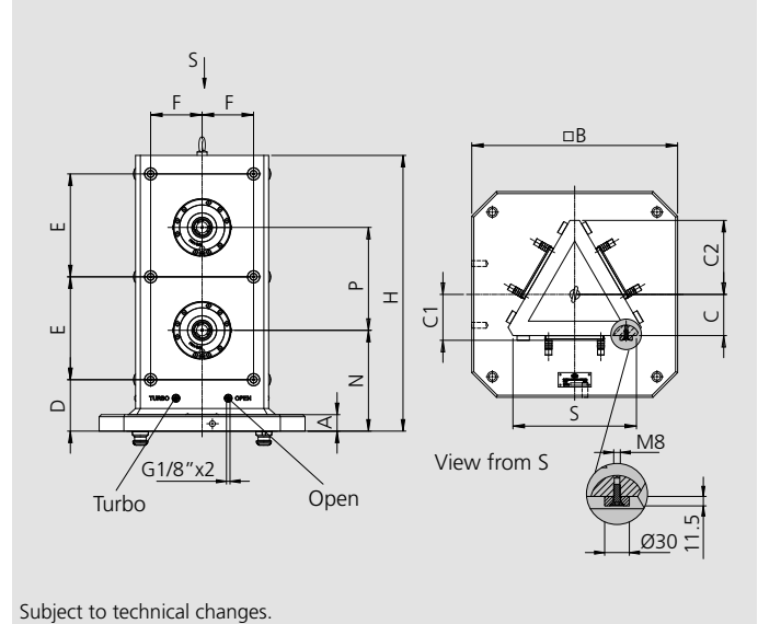
Tombstone with 6 APS modules
