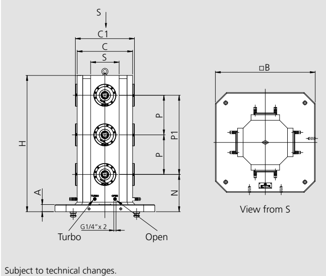
Tombstone with 12 APS modules
